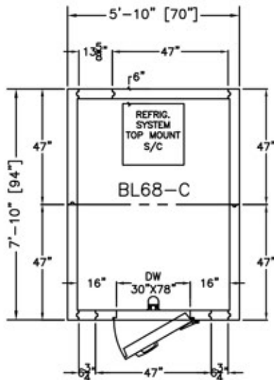
PLAN VIEW
