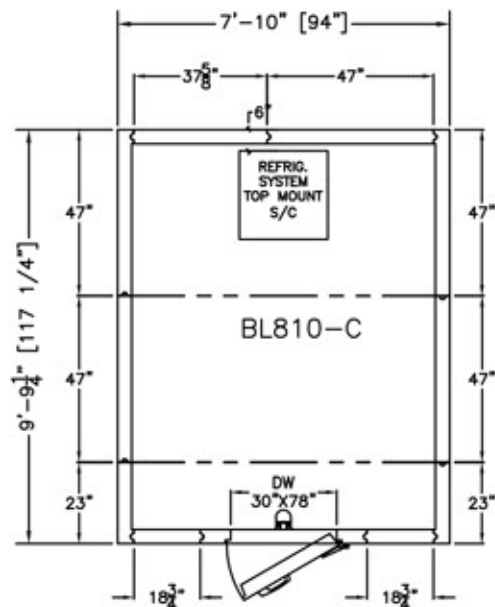
PLAN VIEW
