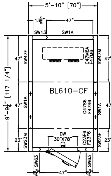
PLAN VIEW
