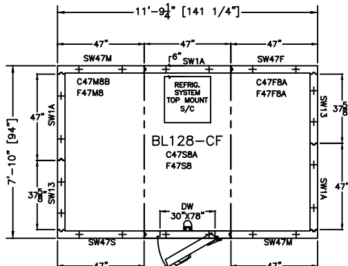
PLAN VIEW
